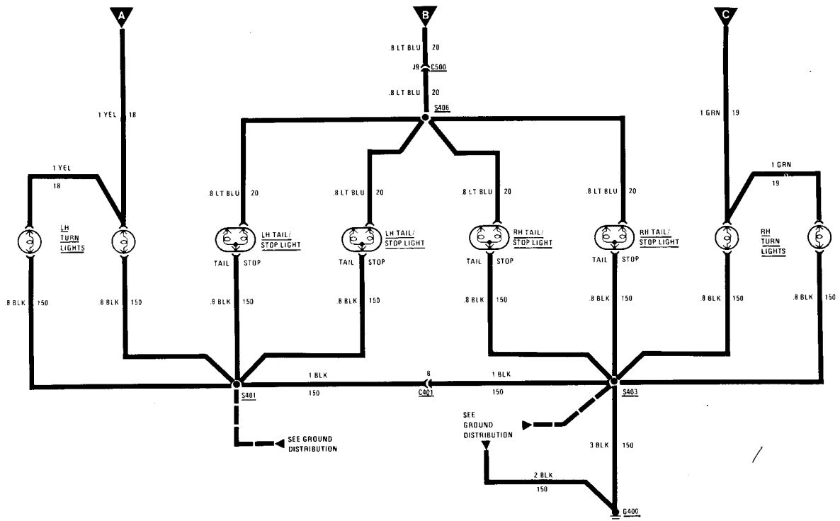
Exterior lights — turn, hazard, park and stop (GT models only)
