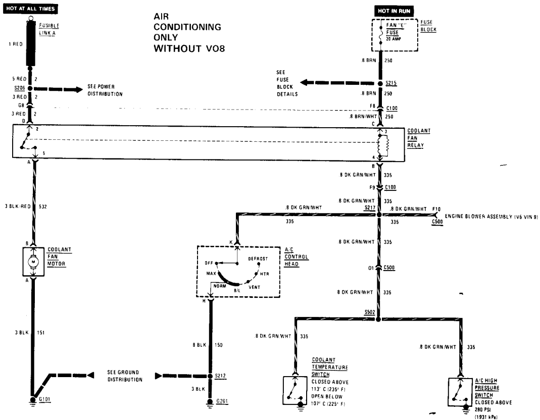
Coolant fan — single-speed (V6 engine)
