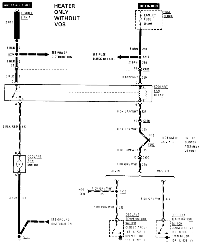
Coolant fan — single-speed (four-cylinder or V6 engine)
