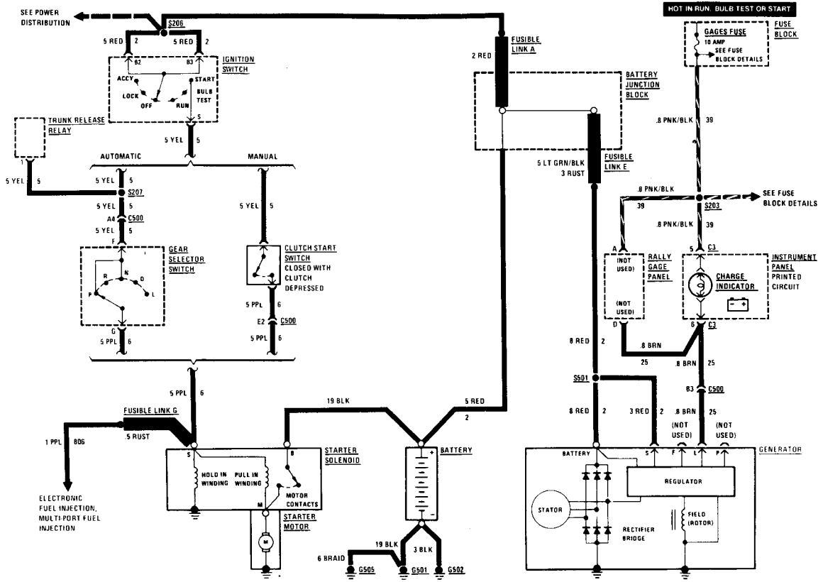
Starter and charging system (four-cylinder engine)
