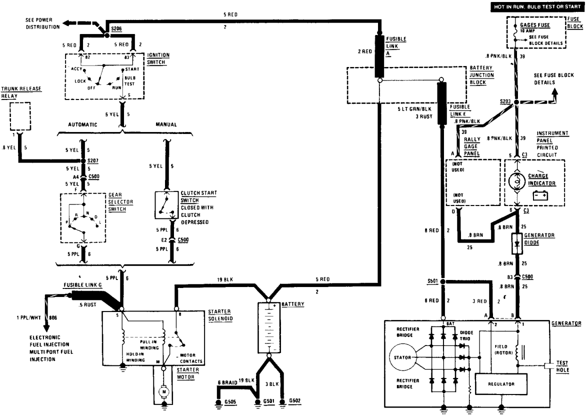
Starter and charging system (V6 engine)
