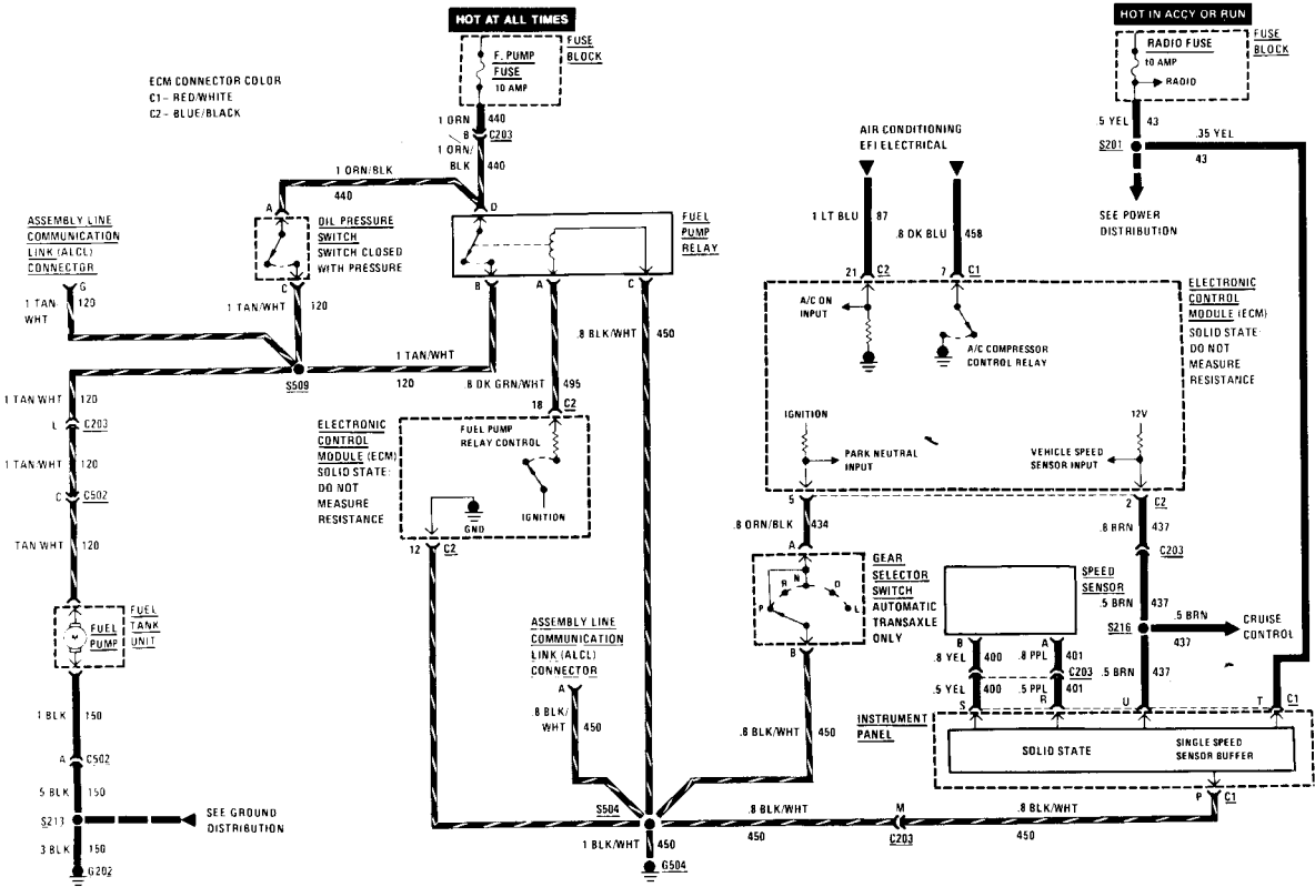
Electronic fuel injection (four-cylinder engine) – fuel control
