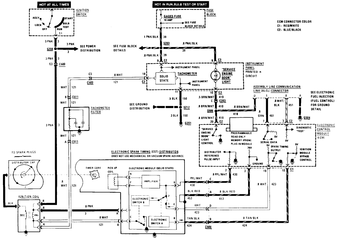
Electronic fuel injection (four-cylinder engine) – ignition, Service Engine Soon light and tachometer
